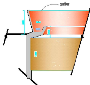
WATERFALL DETAIL
