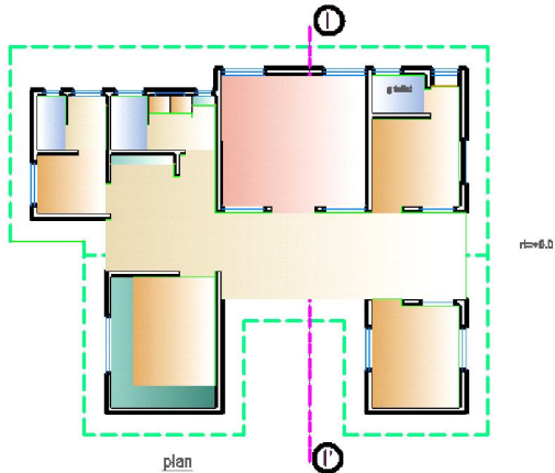
ADMINISTRATION BUILDING
