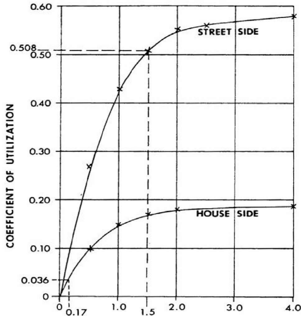
FIGURE F . EXAMPLE OF COEFFICIENT OF UTILIZATION CURVES FOR LUMINAIRE PROVIDING TYPE III - M LIGHT DISTRIBUTION. TYPE I, II, III, IV, & V TO BE OBTAINED FROM MANUFACTURER'S PERFORMANCE DATA
